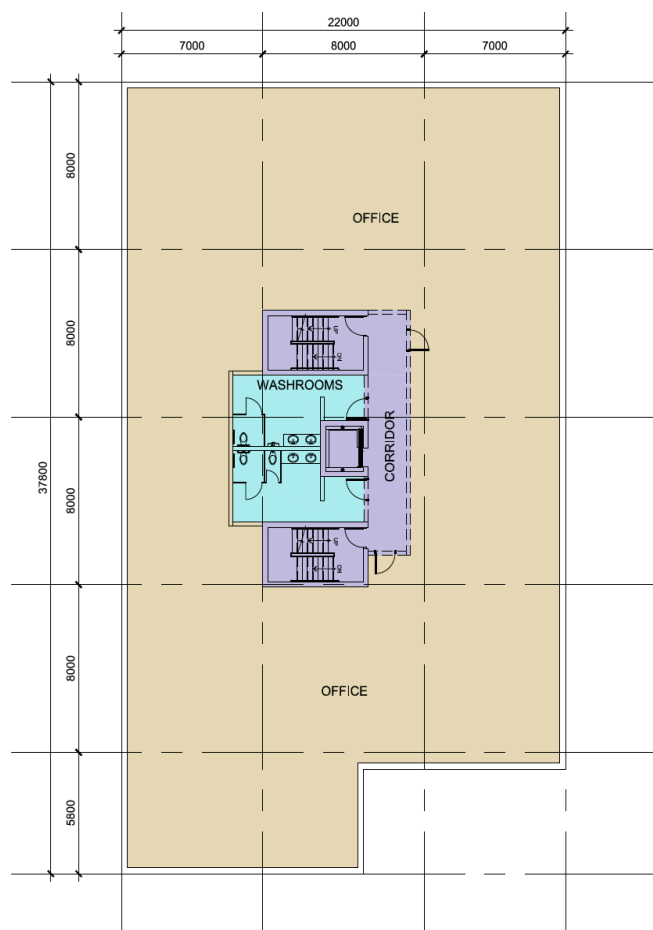
2nd-3rd FLOOR PLAN
